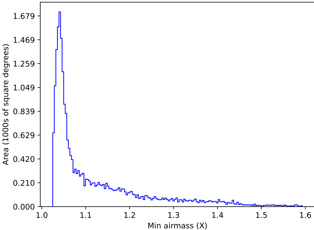
weather_cloudso36v3.4_10yrs All sky u band: Min airmass
