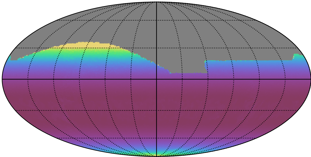
weather_cloudso36v3.4_10yrs All sky r band: Min airmass
