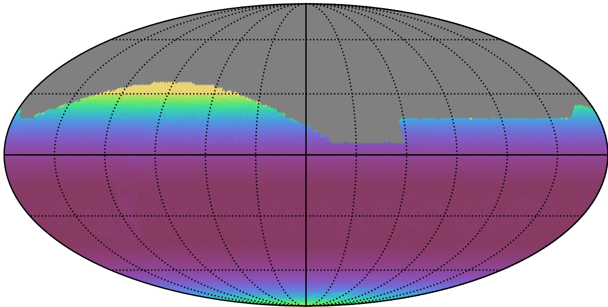
weather_cloudso36v3.4_10yrs All sky i band: Min airmass
