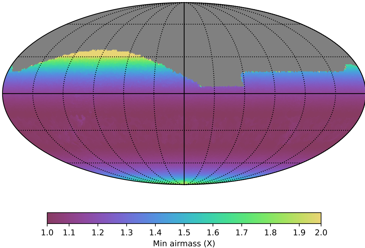
weather_cloudso36v3.4_10yrs All sky g band: Min airmass
