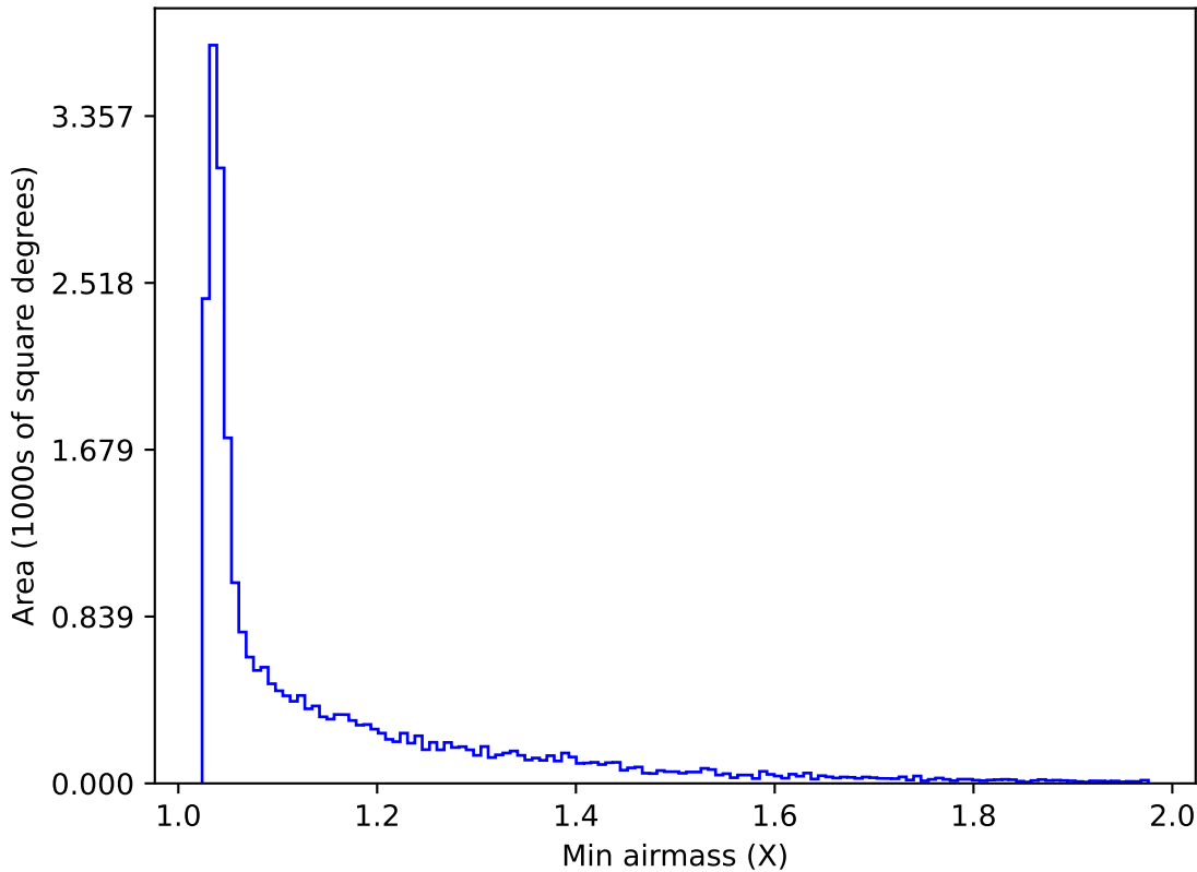
weather_cloudso36v3.4_10yrs All sky g band: Min airmass
