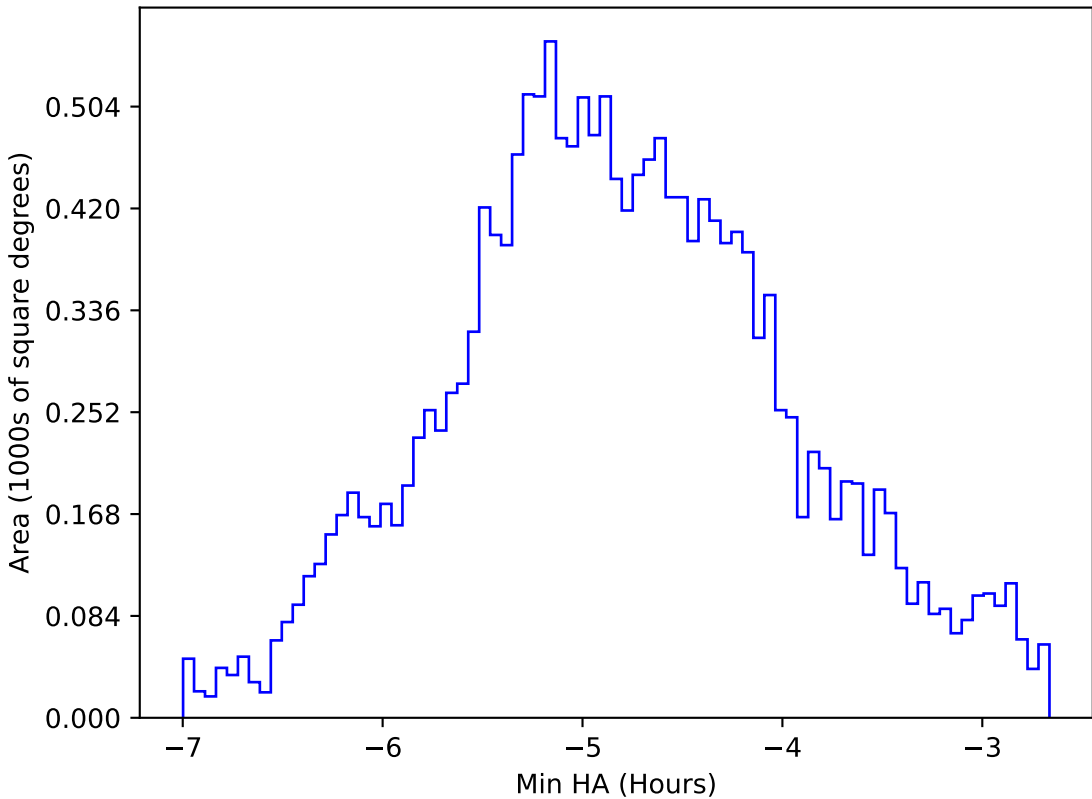
weather_cloudso36v3.4_10yrs WFD all bands: Min HA
