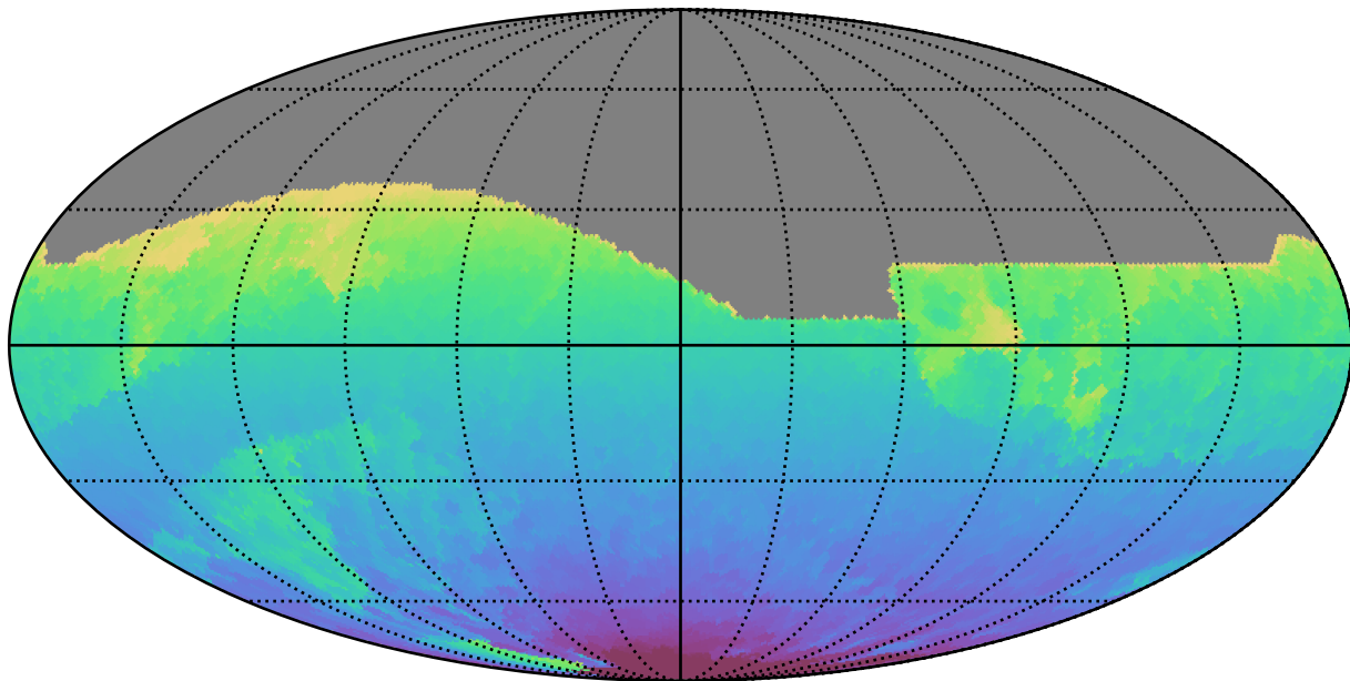
weather_cloudso36v3.4_10yrs All sky all bands: Min HA
