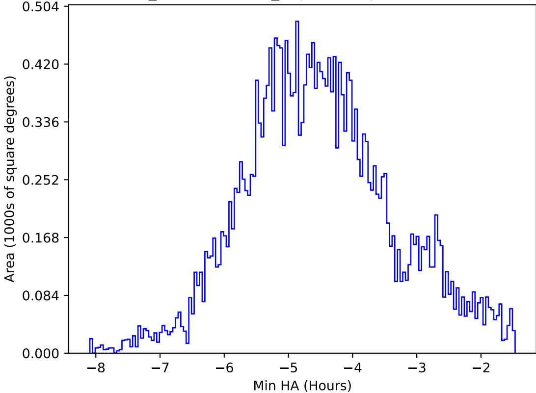
weather_cloudso36v3.4_10yrs All sky all bands: Min HA
