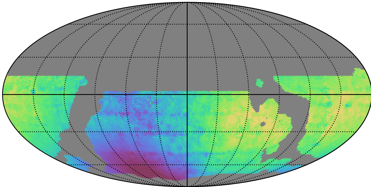
weather_cloudso36v3.4_10yrs WFD z band: Median solarElong
