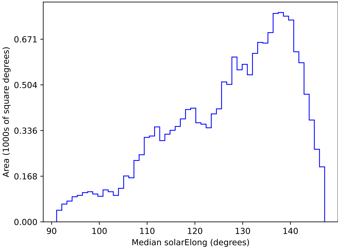
weather_cloudso36v3.4_10yrs WFD z band: Median solarElong
