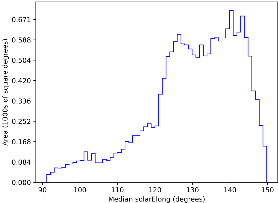
weather_cloudso36v3.4_10yrs WFD r band: Median solarElong
