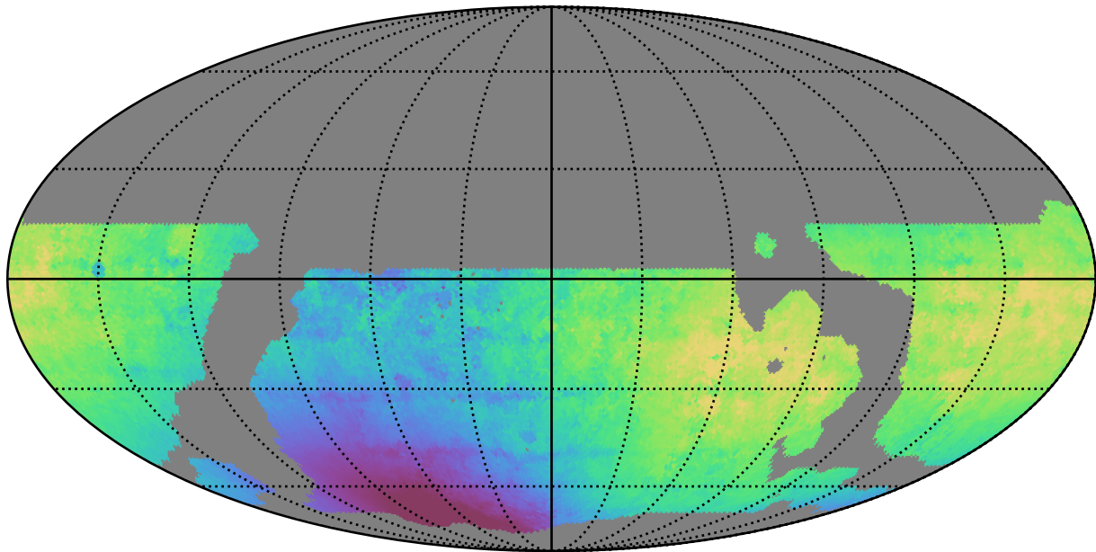
weather_cloudso36v3.4_10yrs WFD i band: Median solarElong
