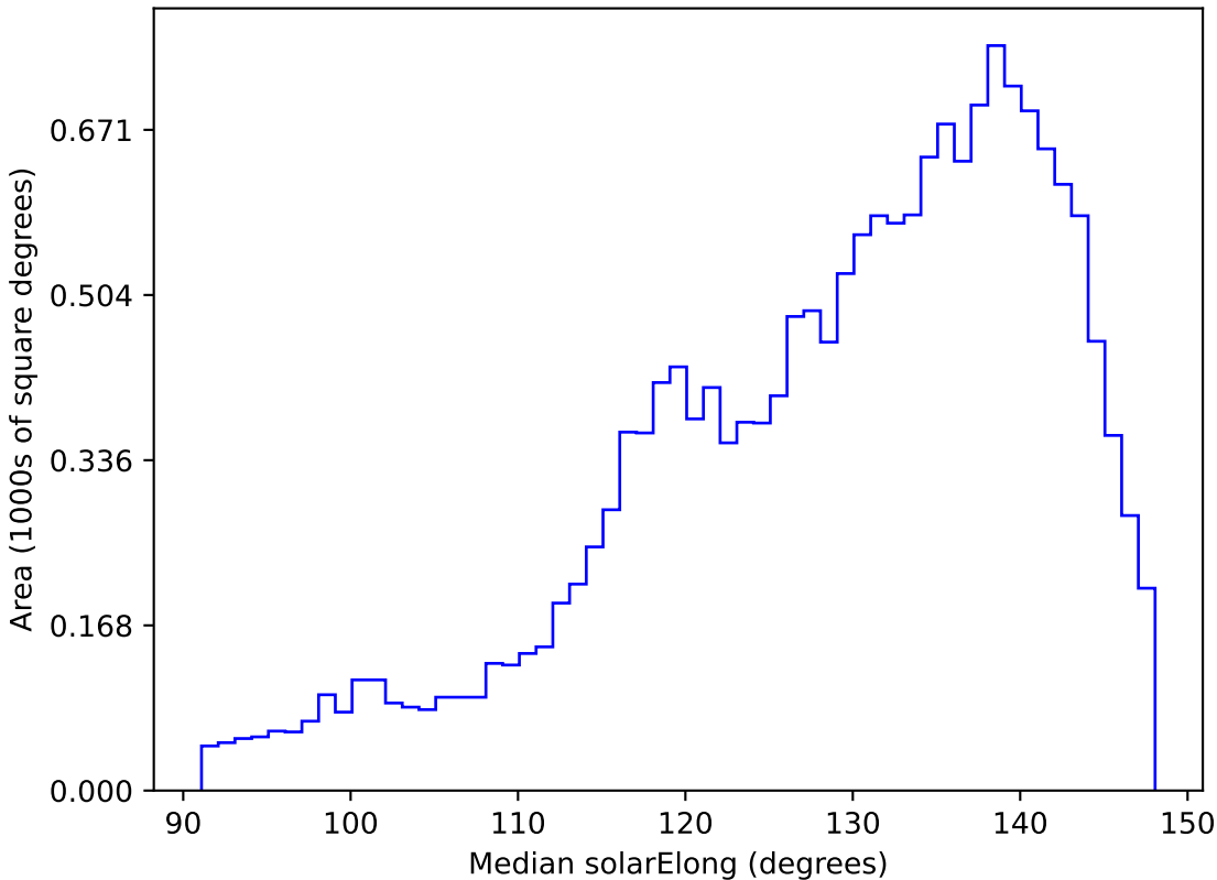
weather_cloudso36v3.4_10yrs WFD i band: Median solarElong
