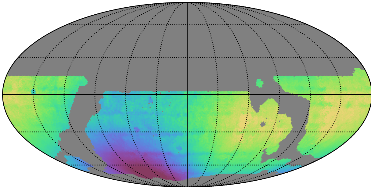
weather_cloudso36v3.4_10yrs WFD all bands: Median solarElong
