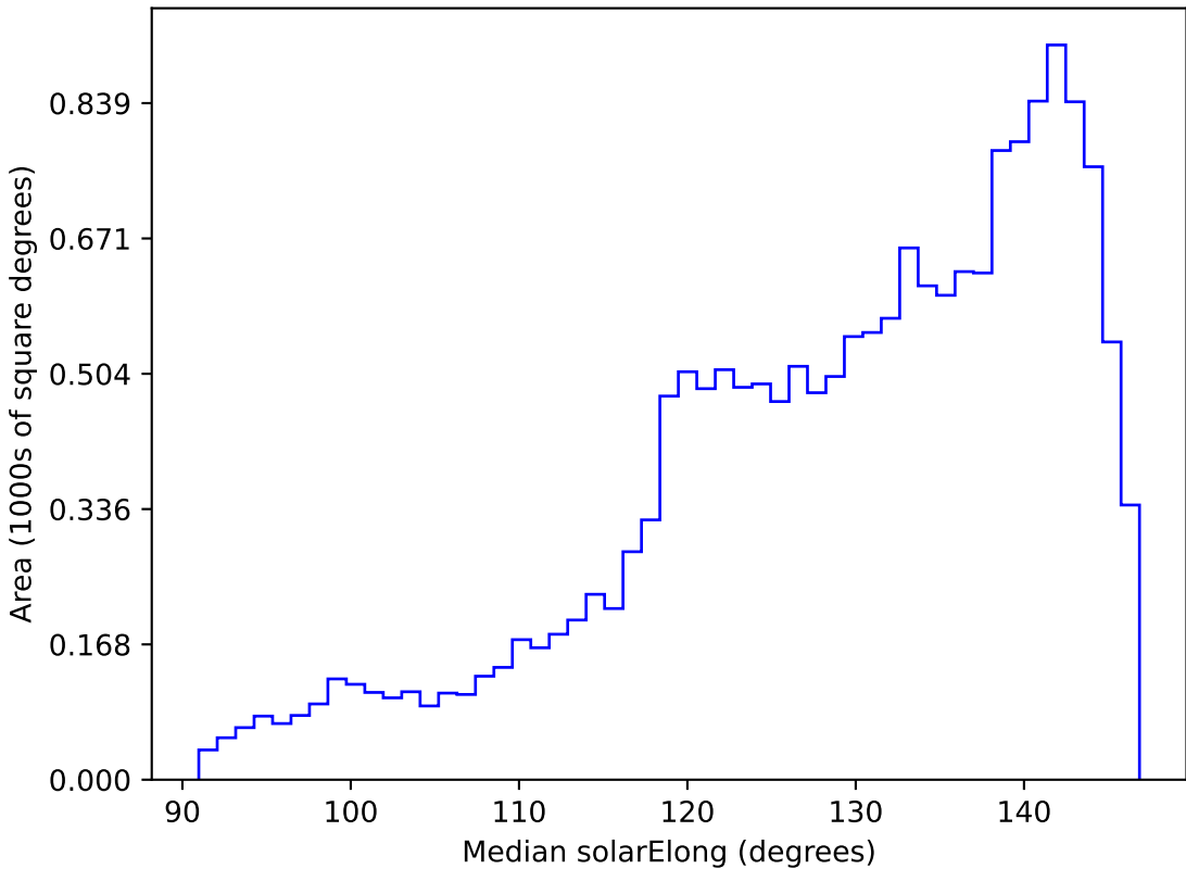
weather_cloudso36v3.4_10yrs WFD all bands: Median solarElong
