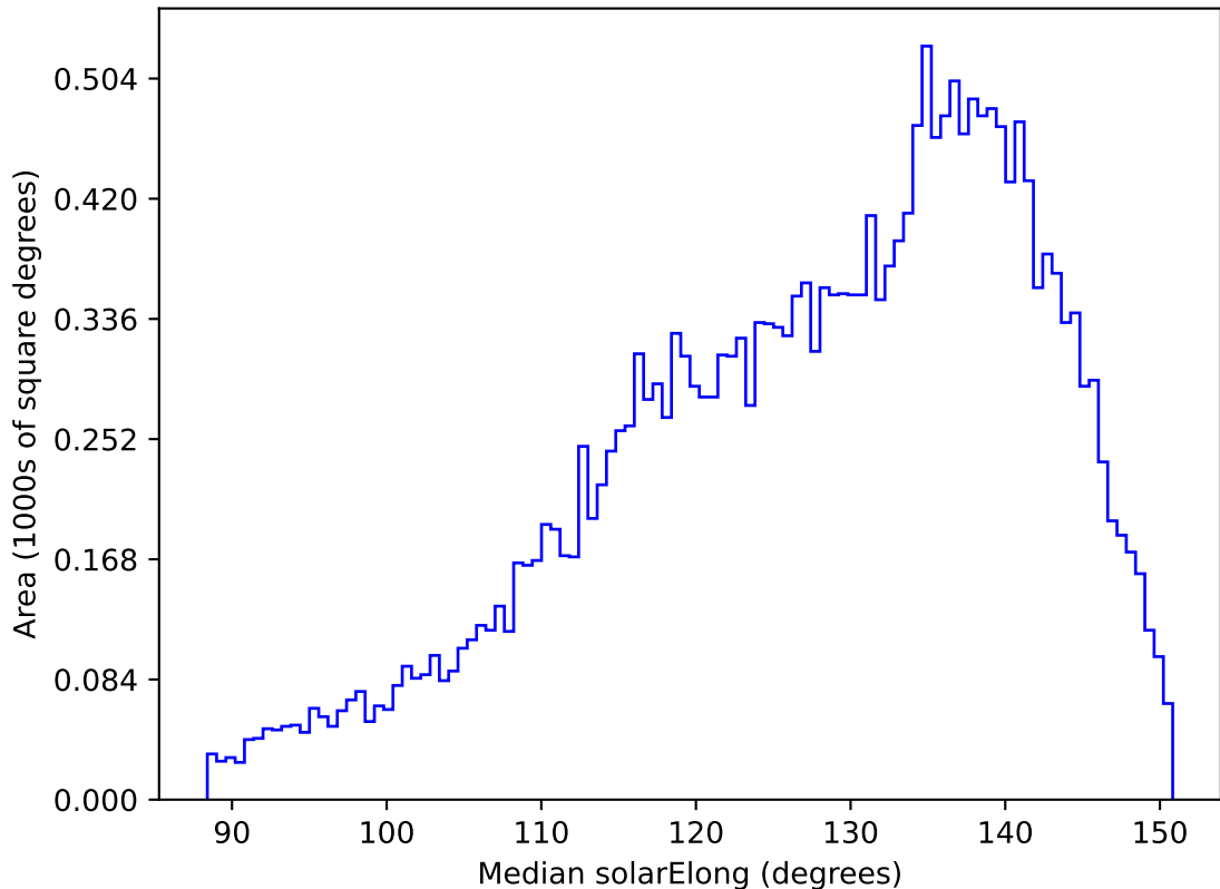
weather_cloudso36v3.4_10yrs All sky y band: Median solarElong
