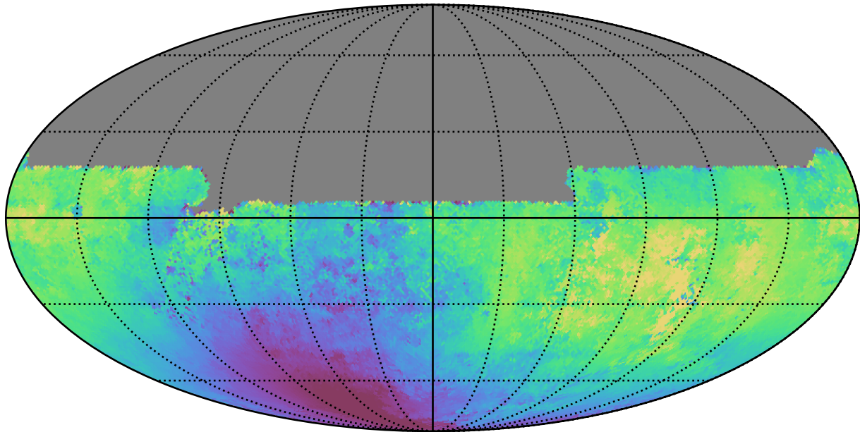
weather_cloudso36v3.4_10yrs All sky u band: Median solarElong
