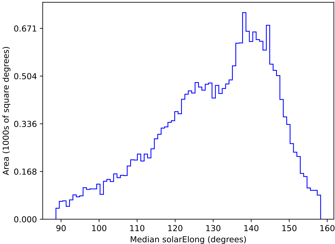
weather_cloudso36v3.4_10yrs All sky u band: Median solarElong
