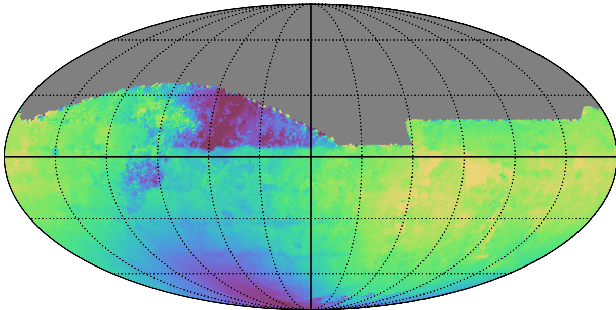
weather_cloudso36v3.4_10yrs All sky i band: Median solarElong
