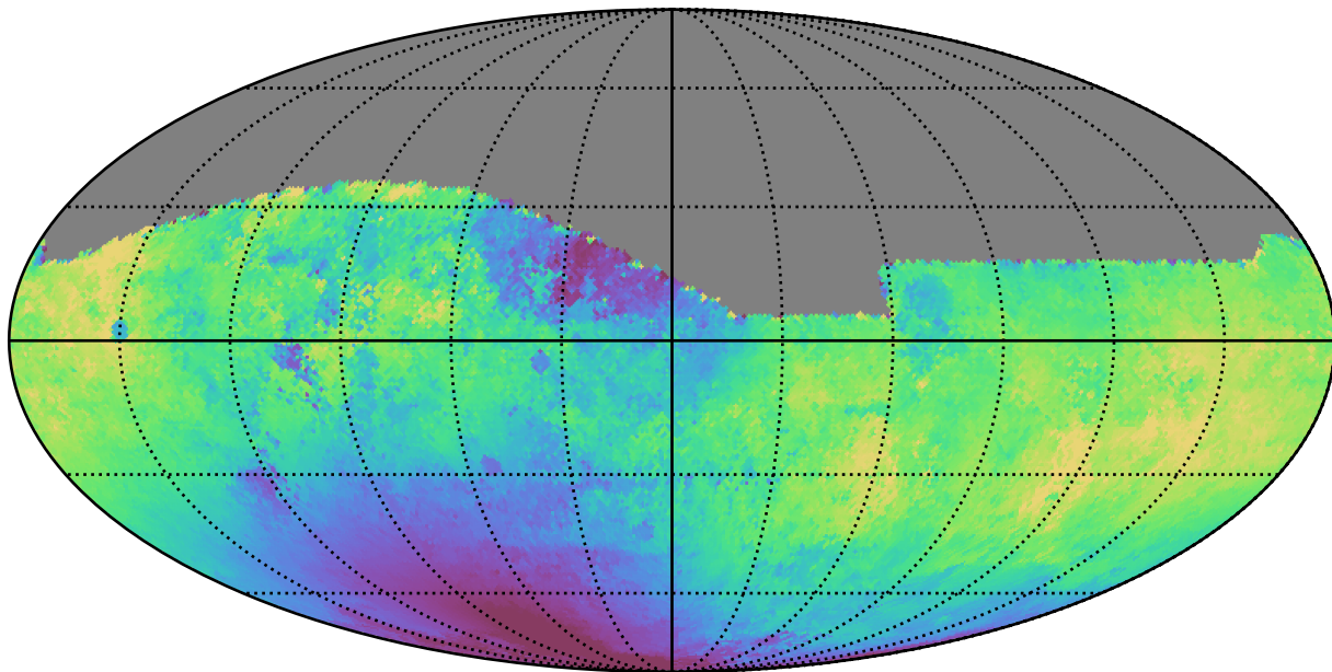
weather_cloudso36v3.4_10yrs All sky g band: Median solarElong
