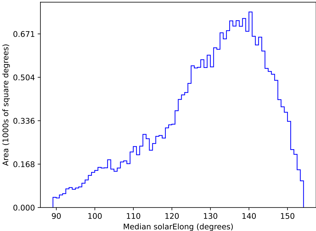
weather_cloudso36v3.4_10yrs All sky g band: Median solarElong
