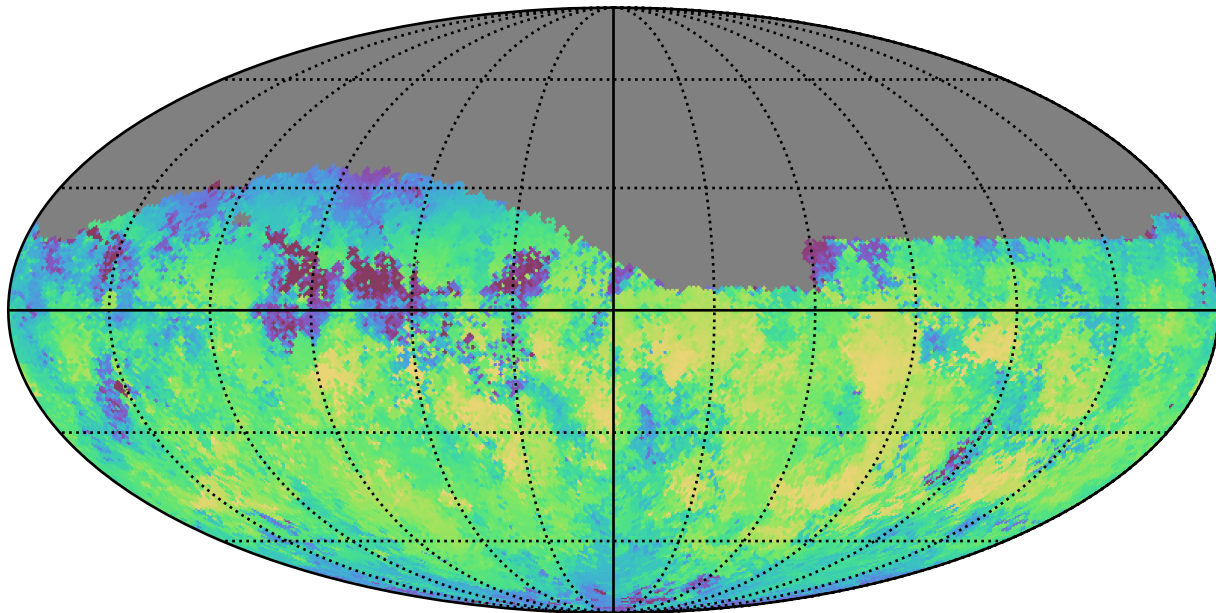
weather_cloudso36v3.4_10yrs Yr 1 z band: Median skyBrightness
