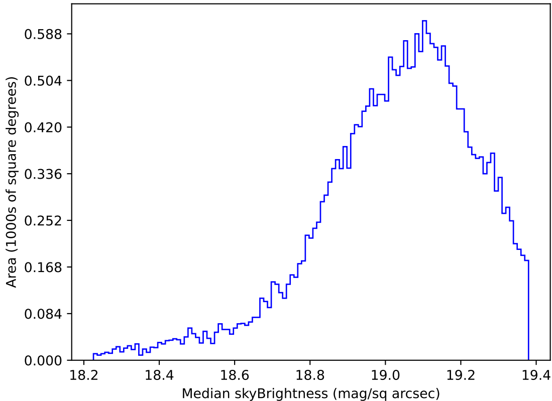
weather_cloudso36v3.4_10yrs Yr 1 z band: Median skyBrightness
