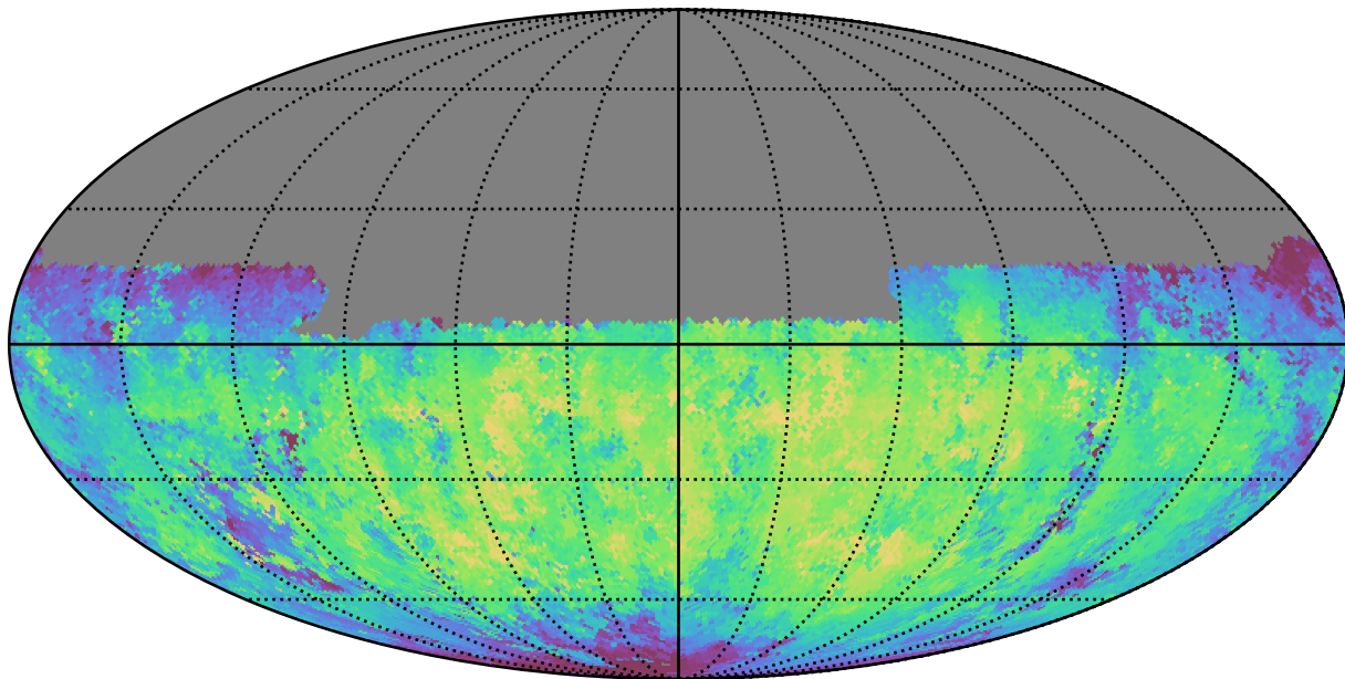
weather_cloudso36v3.4_10yrs Yr 1 y band: Median skyBrightness
