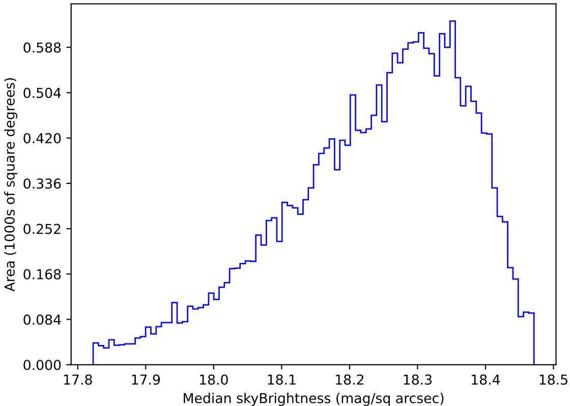
weather_cloudso36v3.4_10yrs Yr 1 y band: Median skyBrightness
