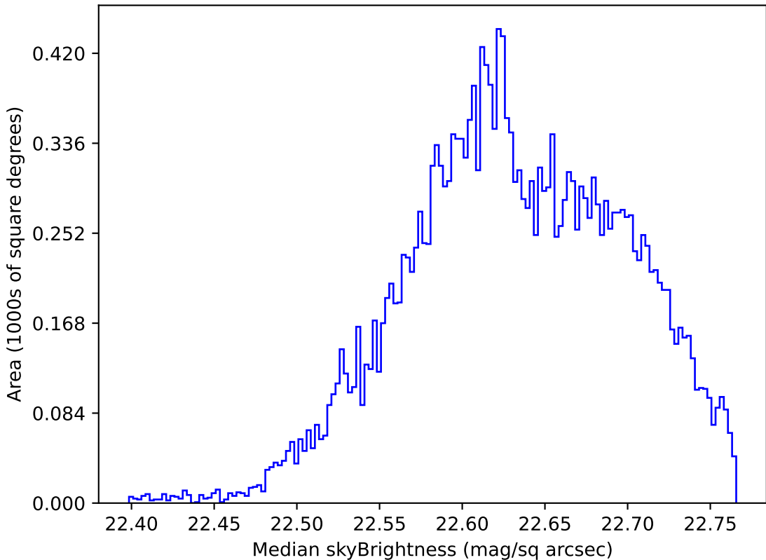
weather_cloudso36v3.4_10yrs Yr 1 u band: Median skyBrightness
