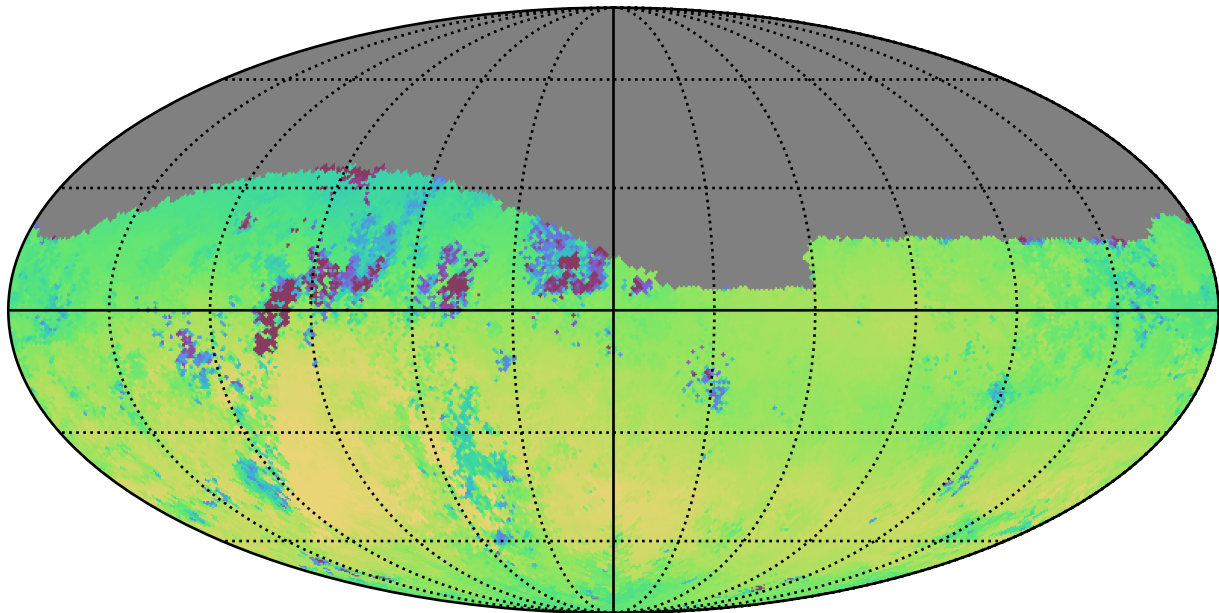
weather_cloudso36v3.4_10yrs Yr 1 r band: Median skyBrightness
