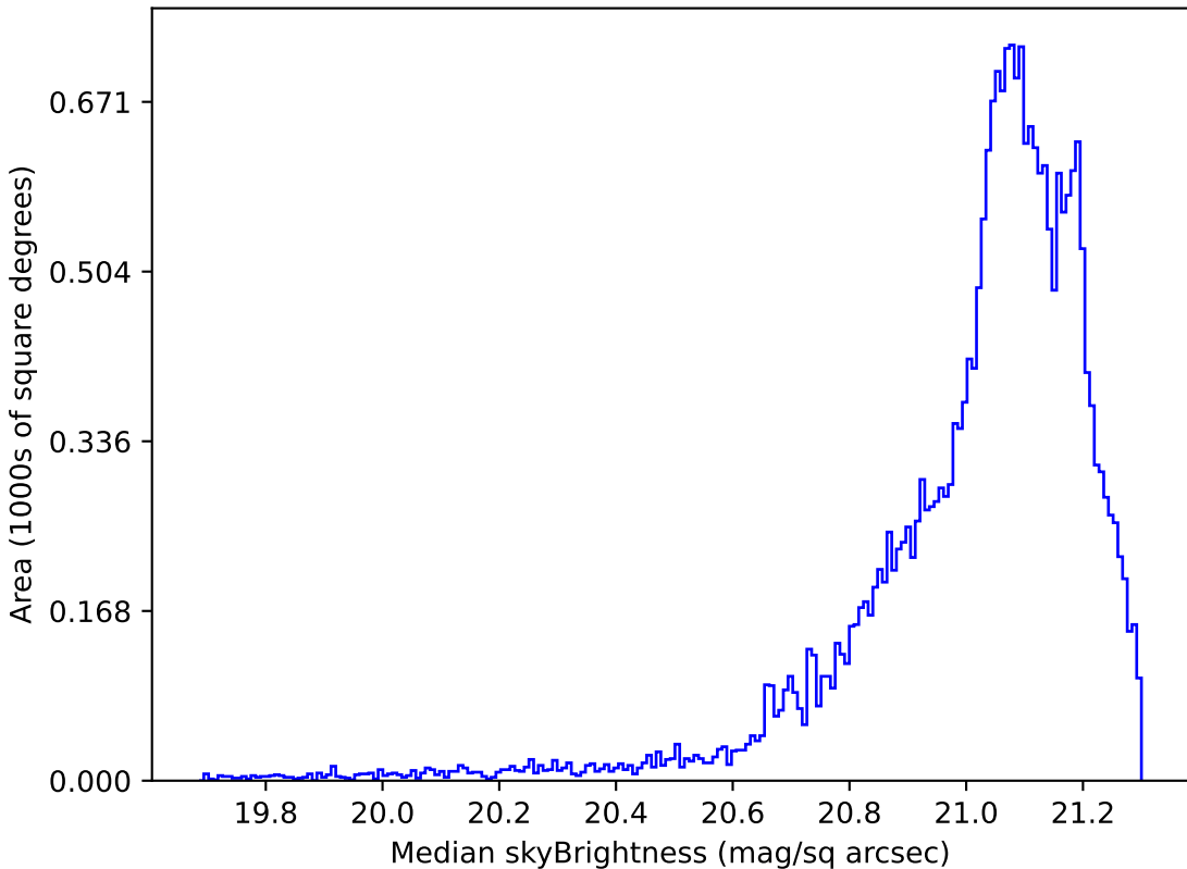
weather_cloudso36v3.4_10yrs Yr 1 r band: Median skyBrightness
