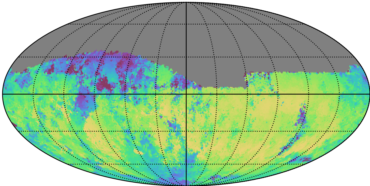
weather_cloudso36v3.4_10yrs Yr 1 i band: Median skyBrightness
