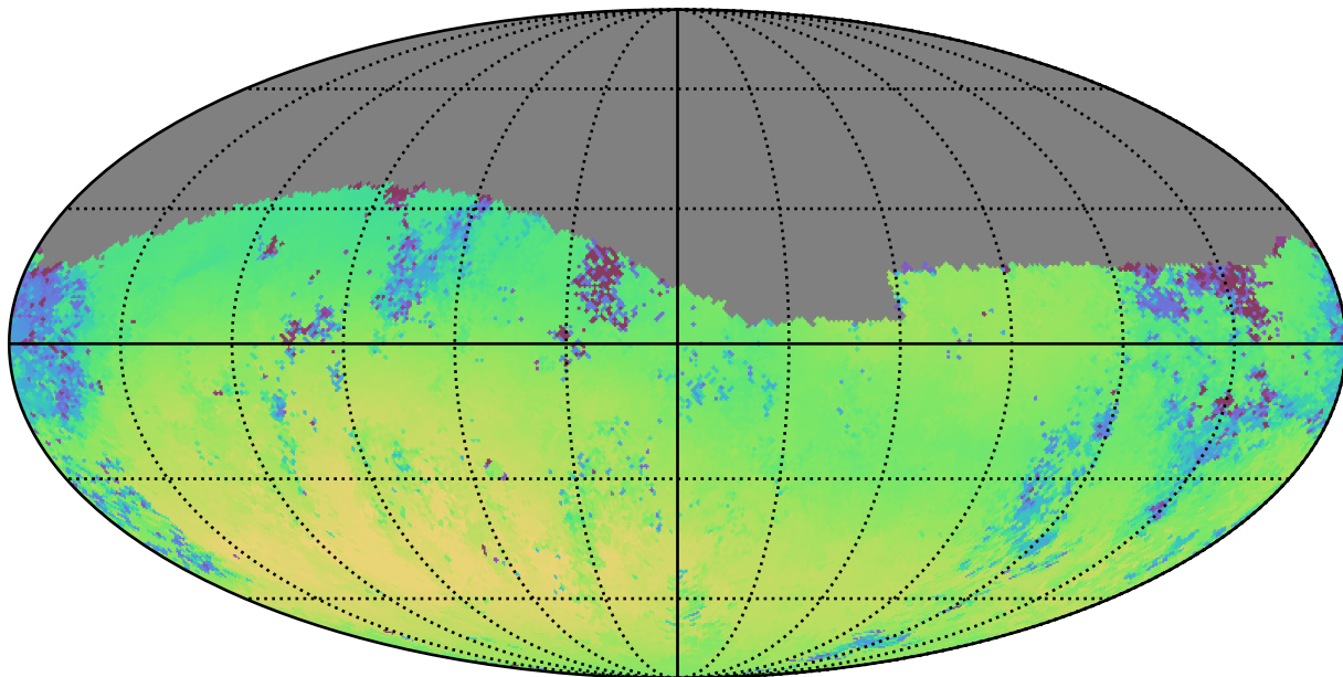
weather_cloudso36v3.4_10yrs Yr 1 g band: Median skyBrightness
