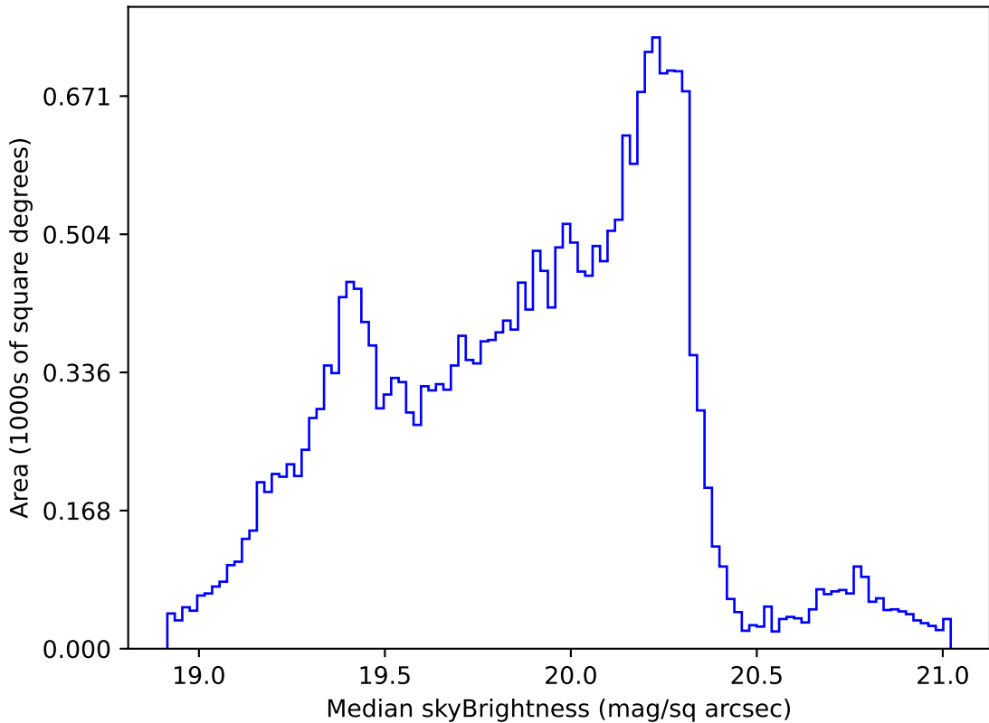
weather_cloudso36v3.4_10yrs Yr 1 all bands: Median skyBrightness
