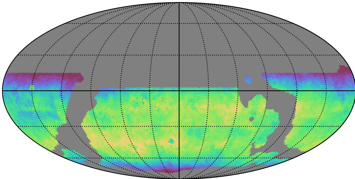
weather_cloudso36v3.4_10yrs WFD y band: Median skyBrightness
