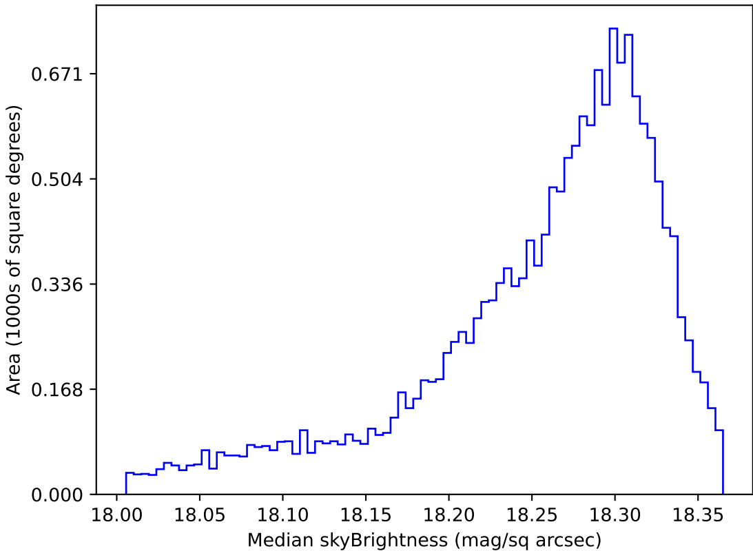
weather_cloudso36v3.4_10yrs WFD y band: Median skyBrightness
