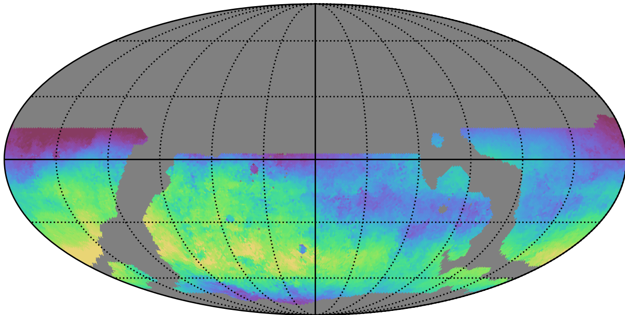
weather_cloudso36v3.4_10yrs WFD u band: Median skyBrightness
