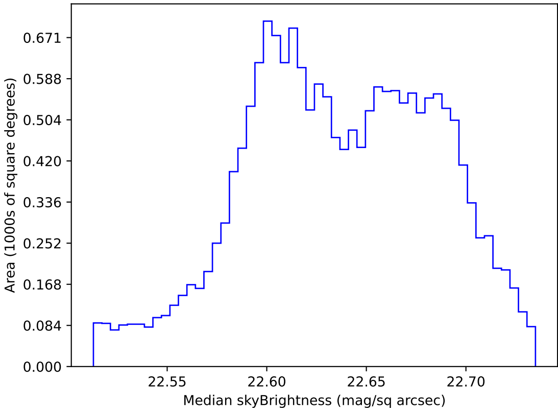
weather_cloudso36v3.4_10yrs WFD u band: Median skyBrightness
