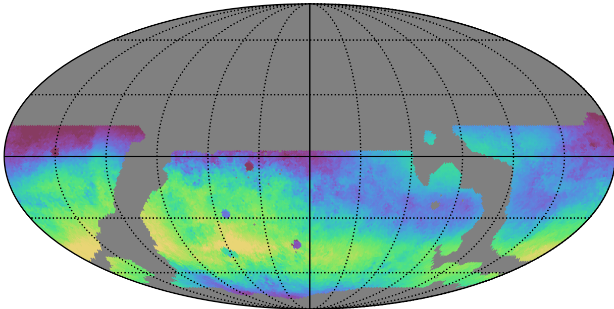
weather_cloudso36v3.4_10yrs WFD r band: Median skyBrightness
