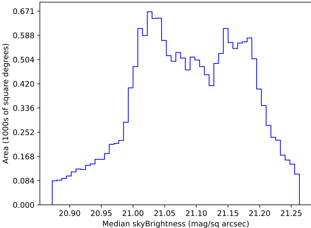
weather_cloudso36v3.4_10yrs WFD r band: Median skyBrightness
