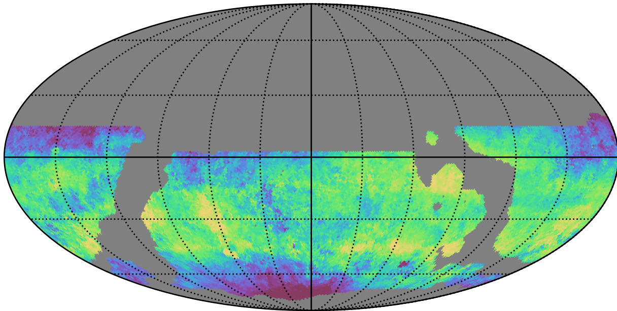
weather_cloudso36v3.4_10yrs WFD i band: Median skyBrightness
