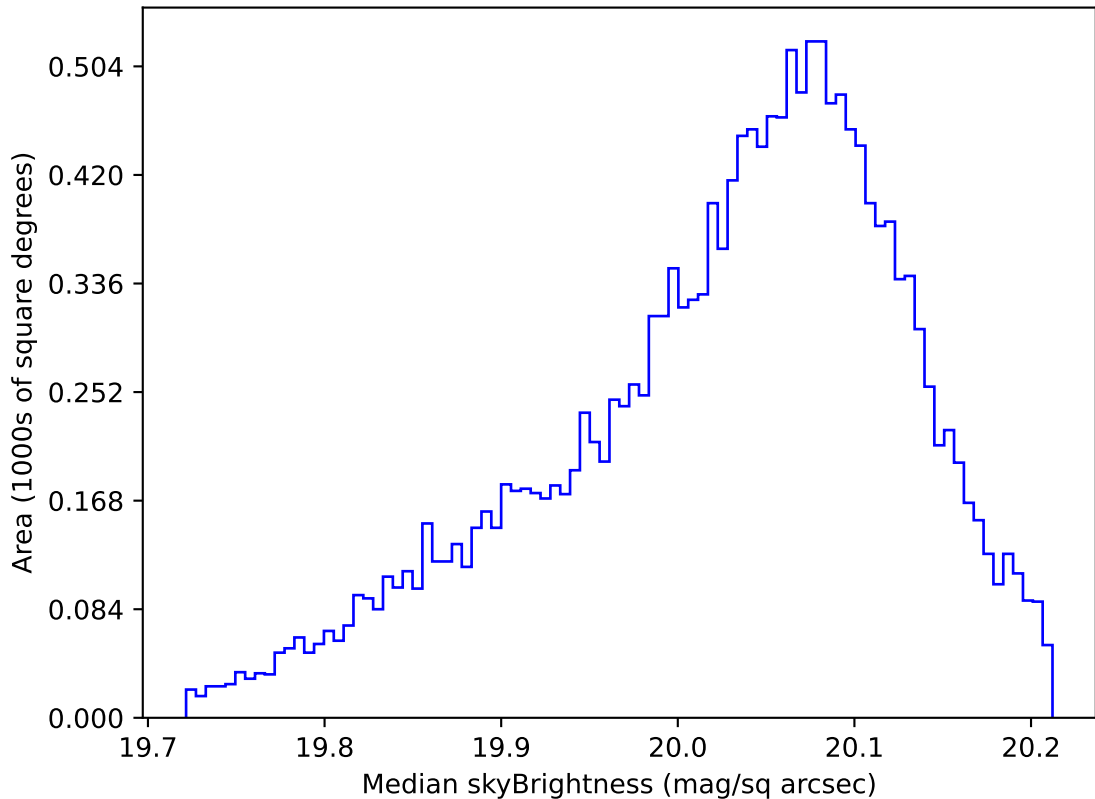
weather_cloudso36v3.4_10yrs WFD i band: Median skyBrightness
