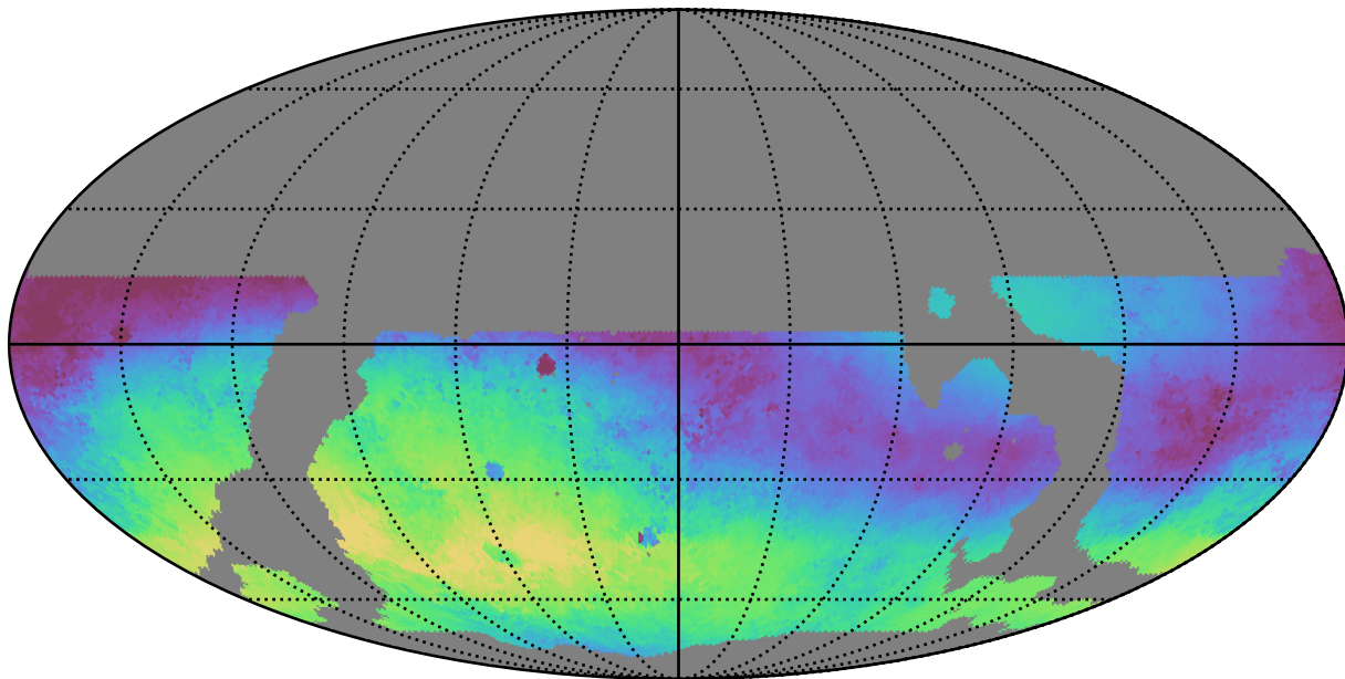
weather_cloudso36v3.4_10yrs WFD g band: Median skyBrightness
