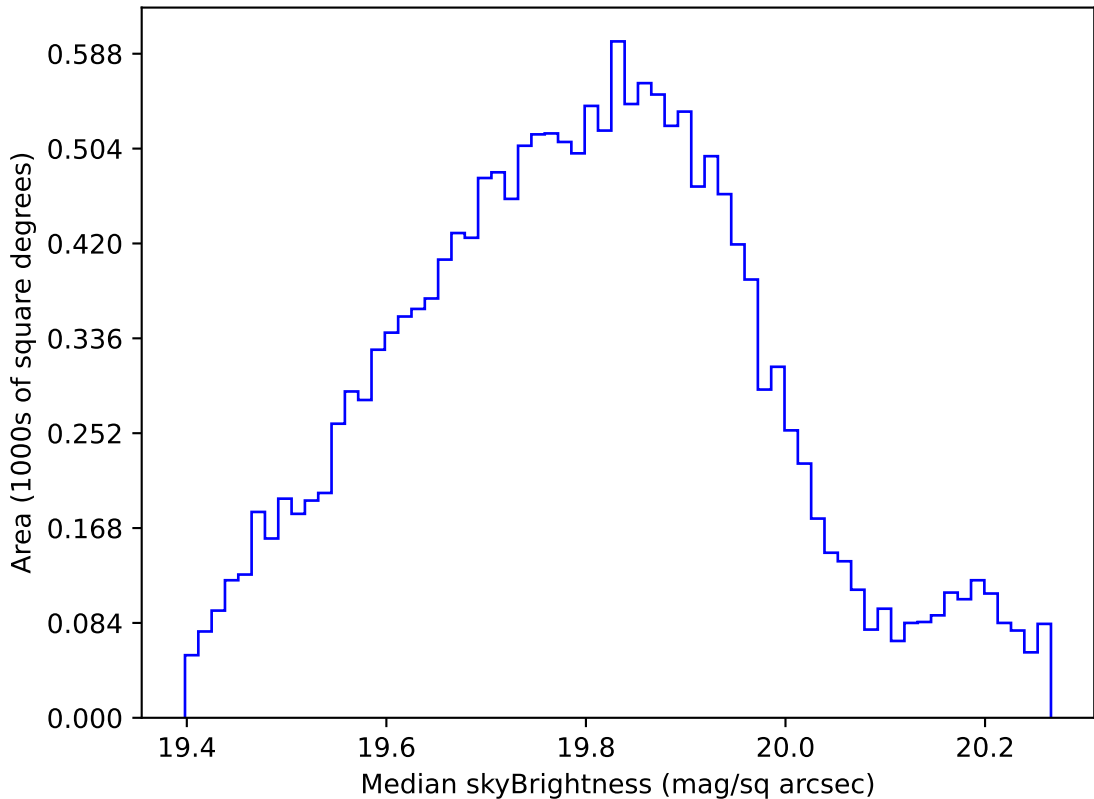
weather_cloudso36v3.4_10yrs WFD all bands: Median skyBrightness
