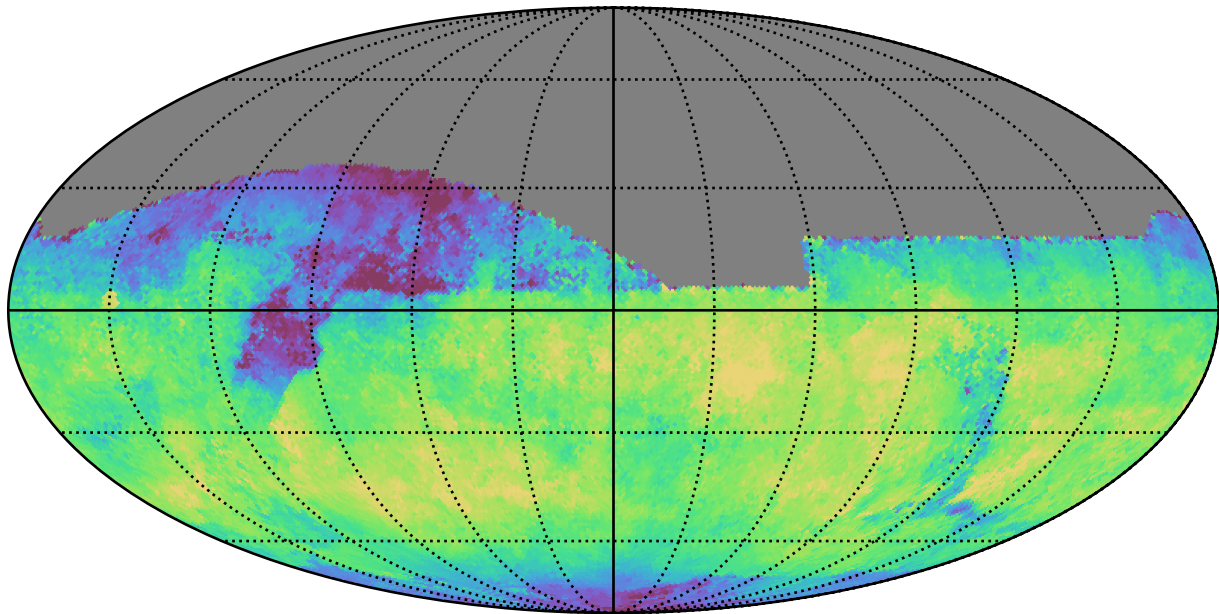
weather_cloudso36v3.4_10yrs All sky z band: Median skyBrightness
