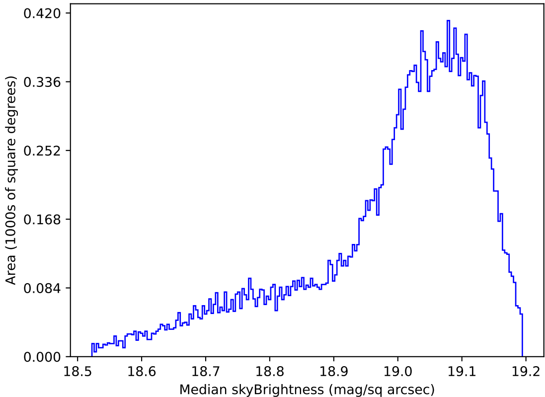
weather_cloudso36v3.4_10yrs All sky z band: Median skyBrightness
