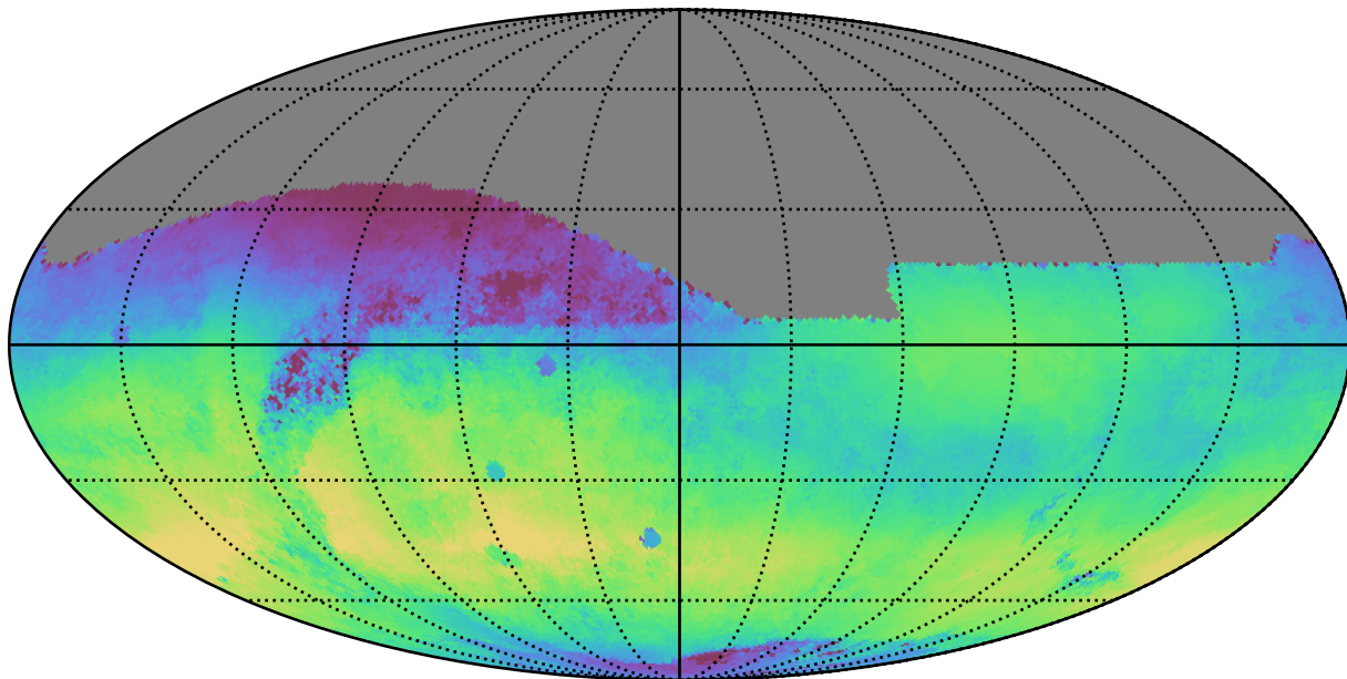
weather_cloudso36v3.4_10yrs All sky r band: Median skyBrightness
