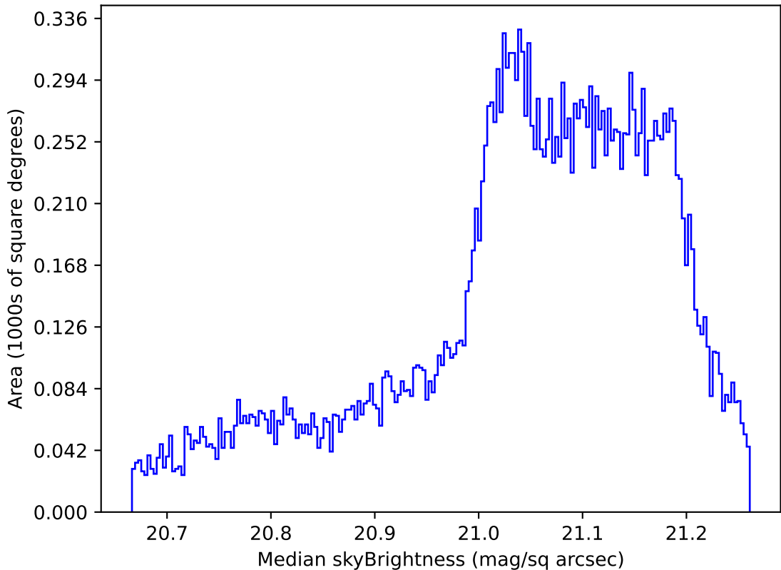
weather_cloudso36v3.4_10yrs All sky r band: Median skyBrightness
