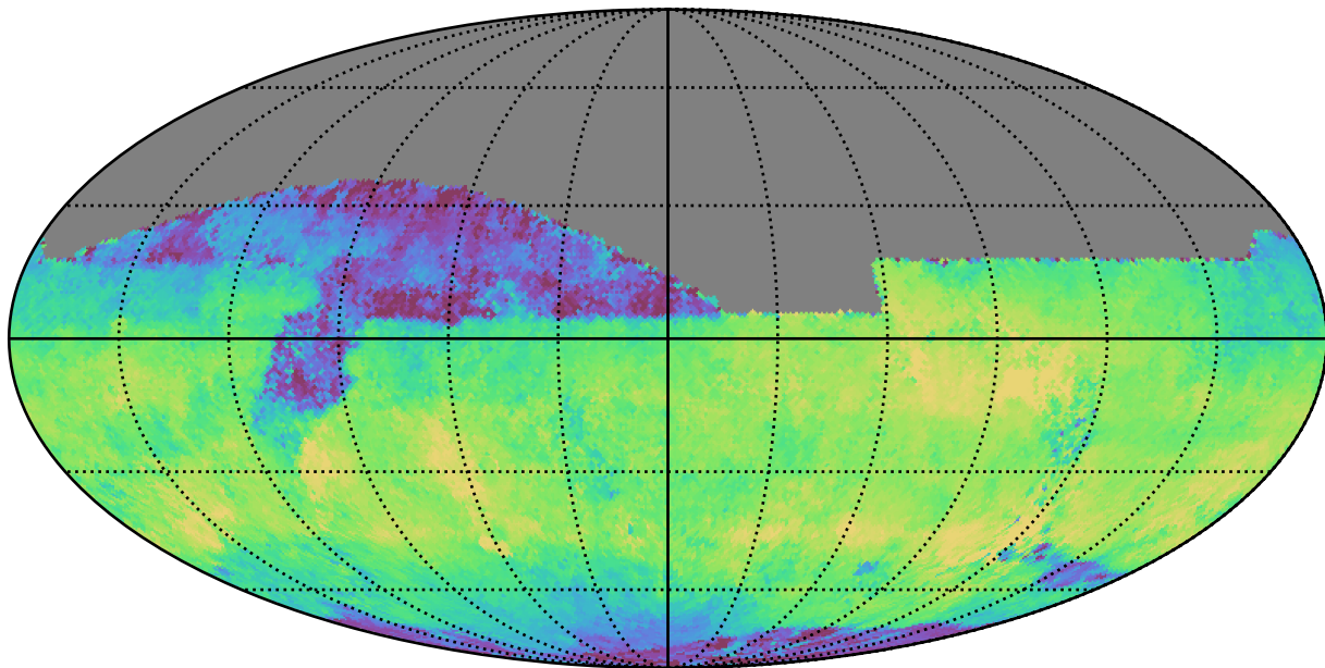
weather_cloudso36v3.4_10yrs All sky i band: Median skyBrightness
