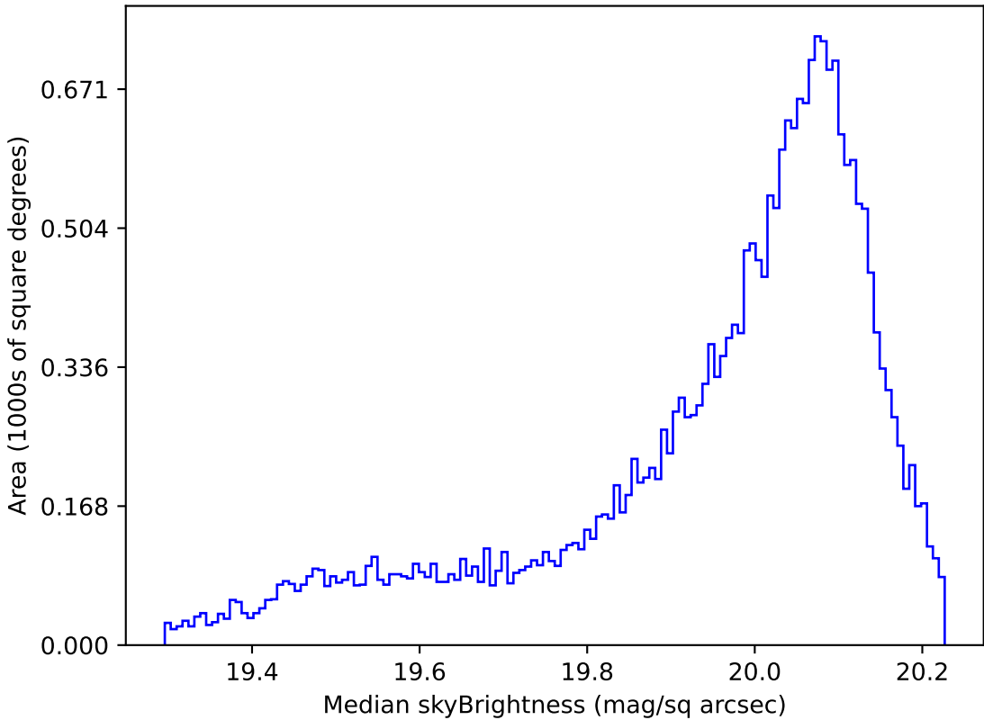
weather_cloudso36v3.4_10yrs All sky i band: Median skyBrightness
