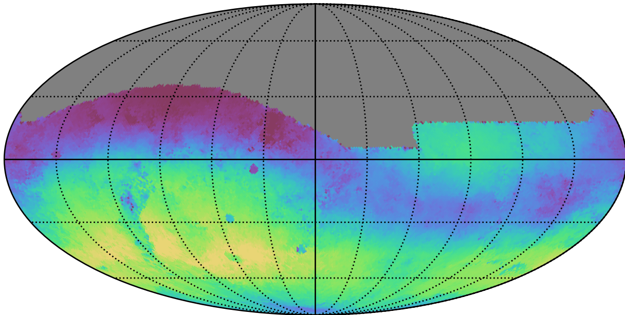
weather_cloudso36v3.4_10yrs All sky g band: Median skyBrightness
