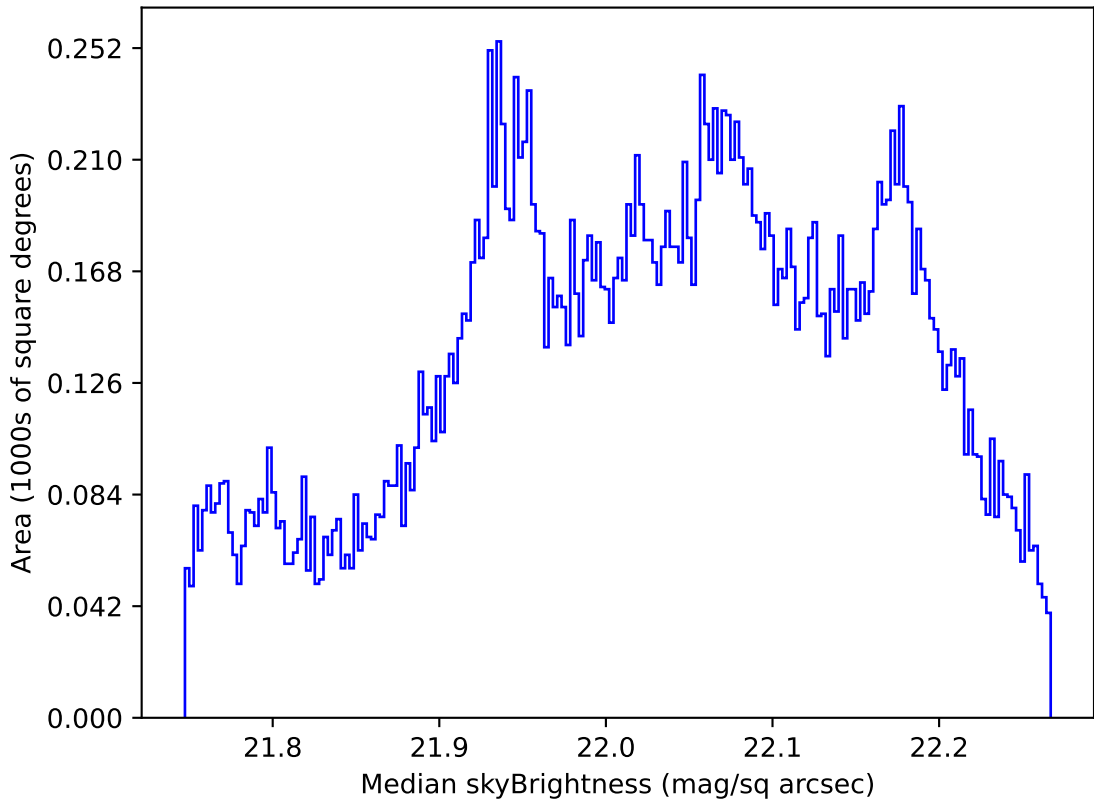
weather_cloudso36v3.4_10yrs All sky g band: Median skyBrightness
