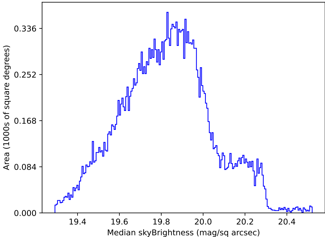
weather_cloudso36v3.4_10yrs All sky all bands: Median skyBrightness
